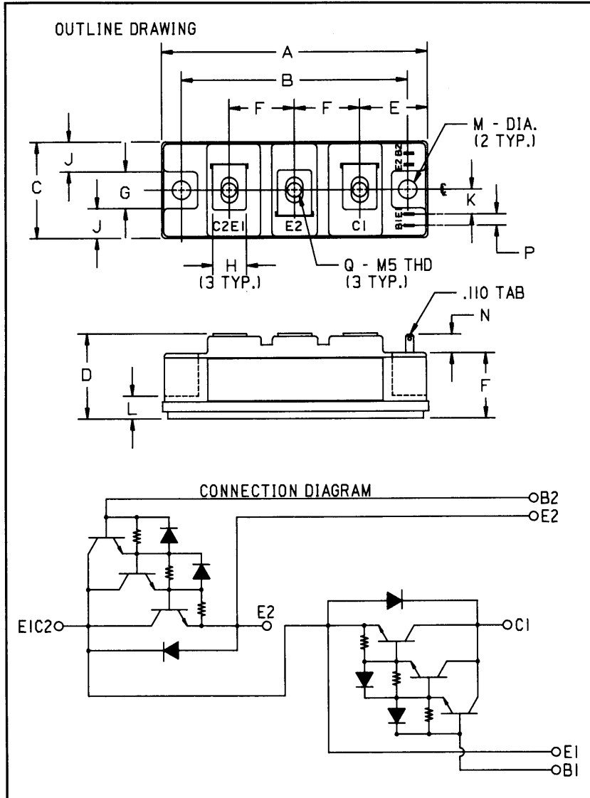
Outline Drawing
