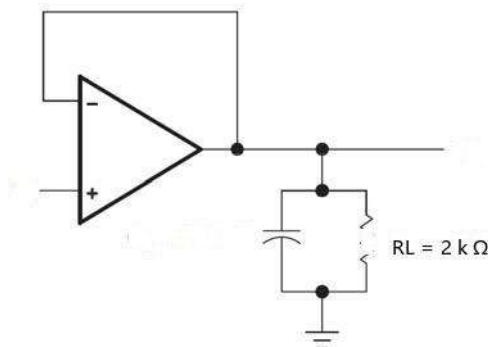
Figure 1. Unity Gain Circuit
