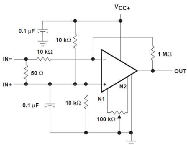
Figure 4. AC amplifier
