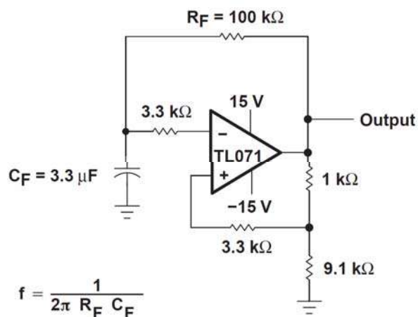
Fig. 5 0.5Hz square wave oscillator
