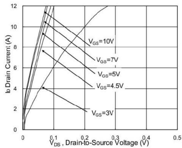
Typical Characteristics
