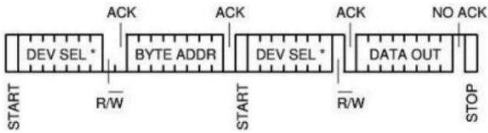
Fig5.IIC read timing diagram
