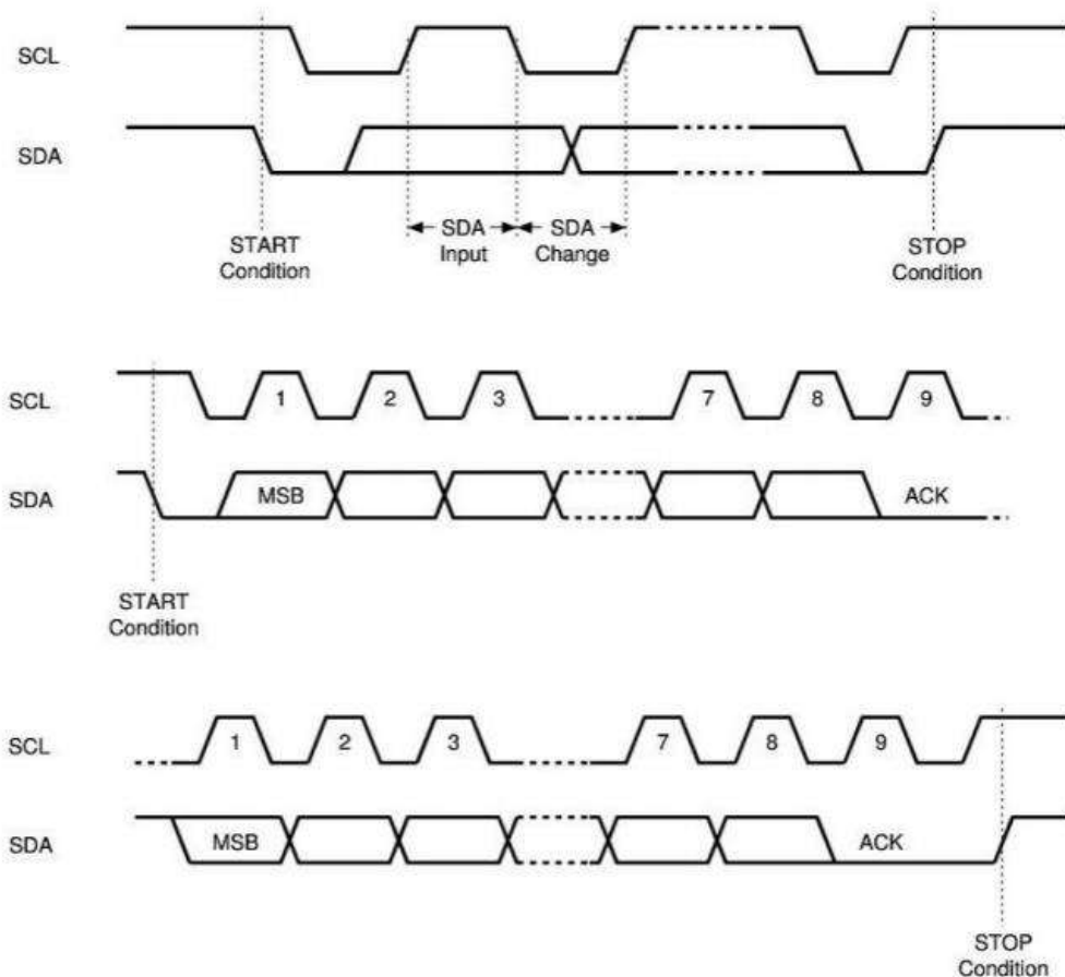
Fig4.IIC communication protocol
