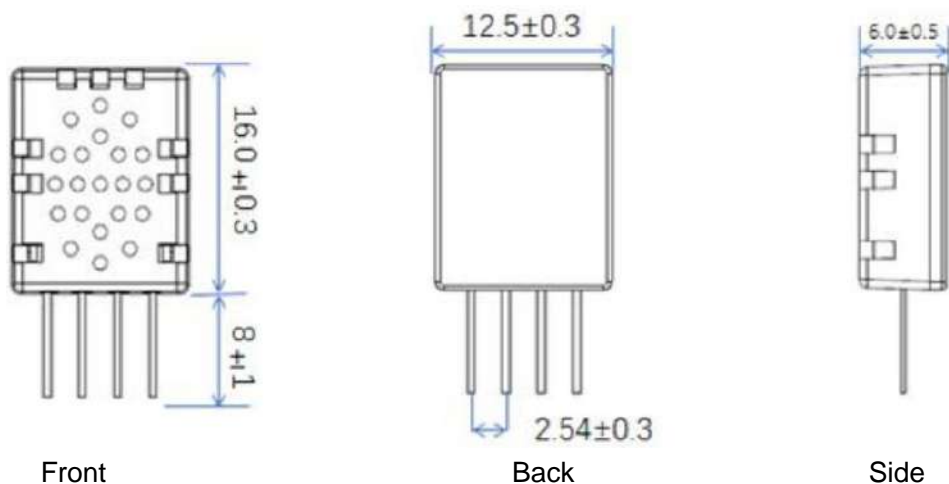
Fig1: Structure
