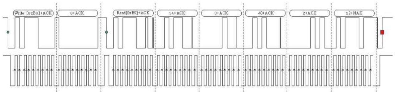
Fig6.Reference timing diagram
