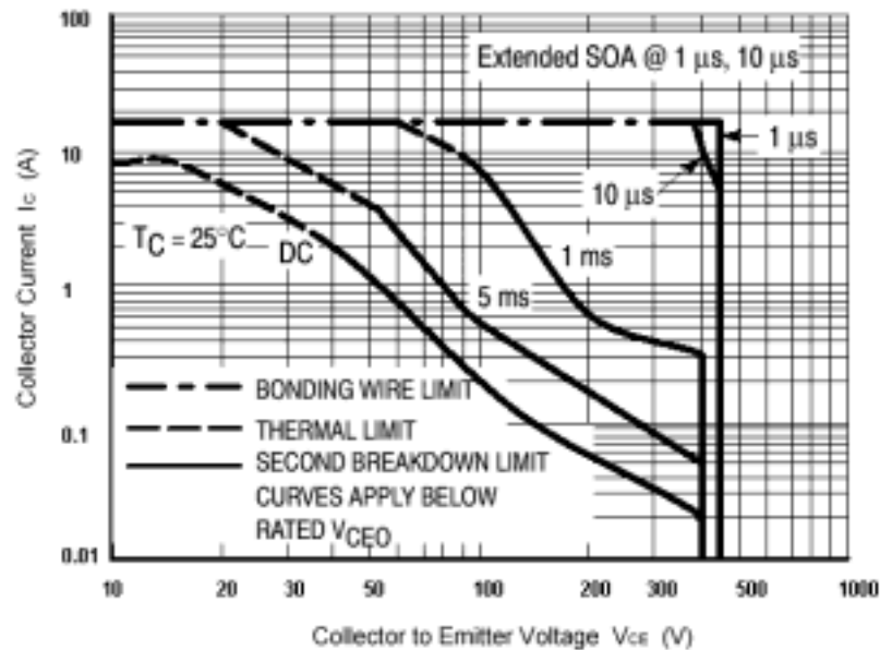
Fig.6 Safe Operating Area
