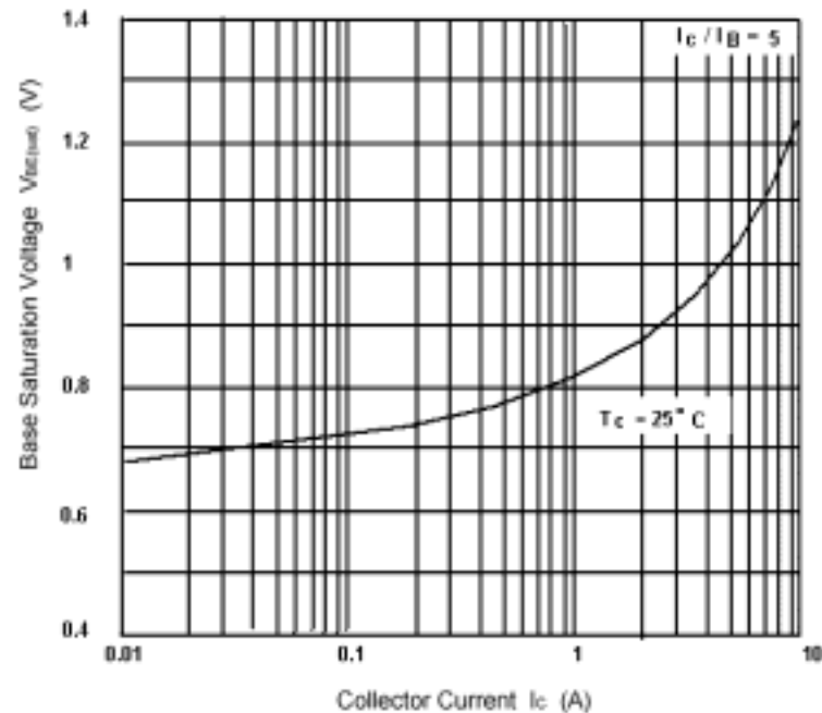
Fig.5 Base-Emitter Saturation Voltage
